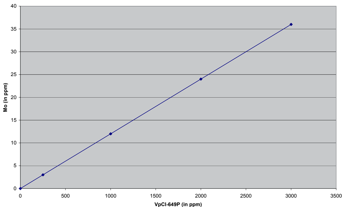
Theoretical concentration of Molybdenum vs. VpCI-649P
